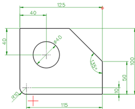
Good Dimensioning
